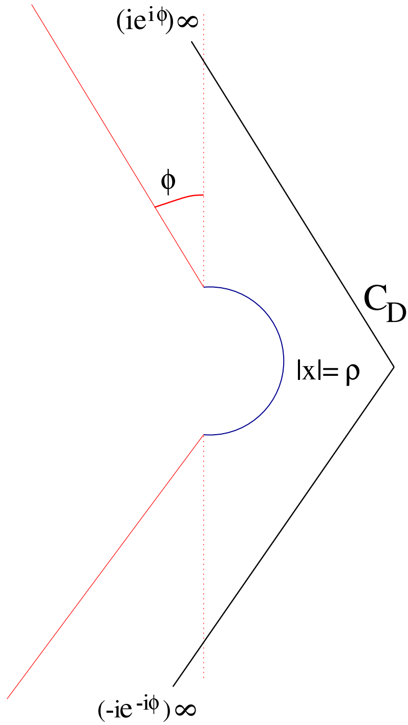
FIGURE 1. Contour C_D in the (\mathbf{p})_i -plane.
