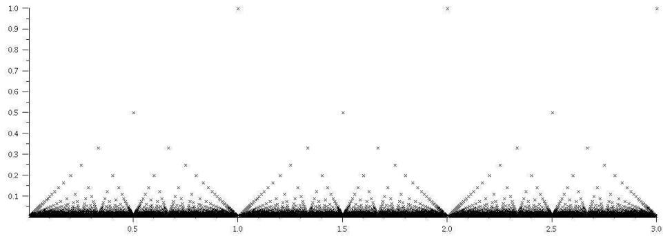
FIGURE 1. The standard function Q(x) . The points above Q = 0.05 are the only ones present in the actual graph.
