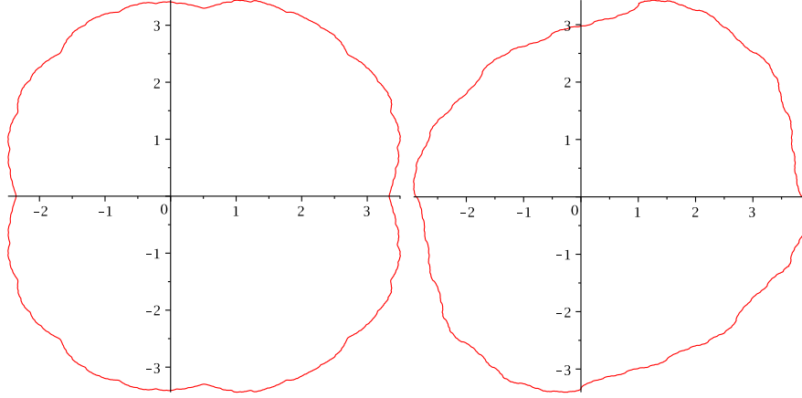
FIGURE 4. The Julia set of x_{n+1} = \lambda x_n(1 - x_n) , for \lambda = 0.3 and \lambda = 0.3i , calculated from the Fourier series (30) discarding all o(\lambda^2) terms. They coincide, within plot precision, with numerically calculated ones using standard iteration of maps algorithms.
