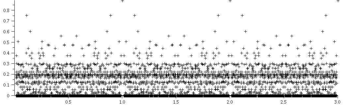
FIGURE 3. Point-plot graph of Q_{3,3} ; Q_{3,2} follows from it through the transformation (24).
