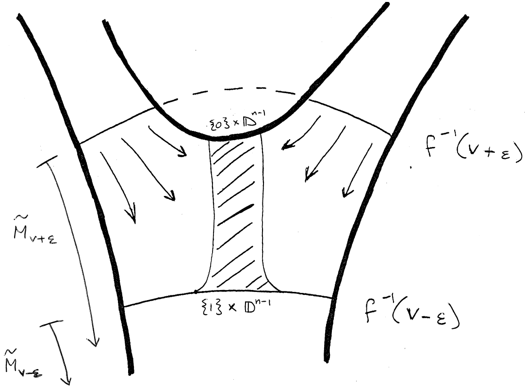
FIGURE 3. Change of topology across a boundary critical point.
