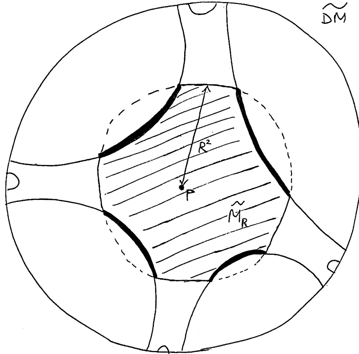
FIGURE 1. Stratified manifold with corners \tilde{M}_R := f^{-1}(-\infty, R] .
