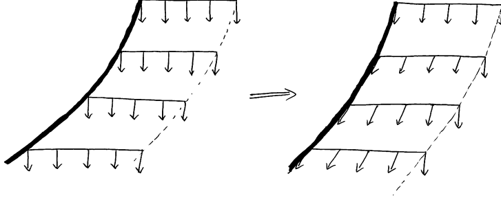
FIGURE 2. Modifying -\nabla f to obtain the vector field X .
