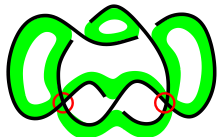
checkerboard colorable
