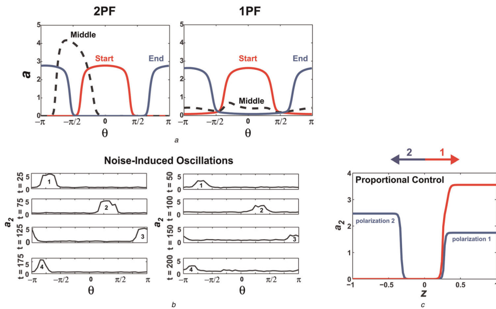
Fig. 3. PDE modelling of mating morphologies
