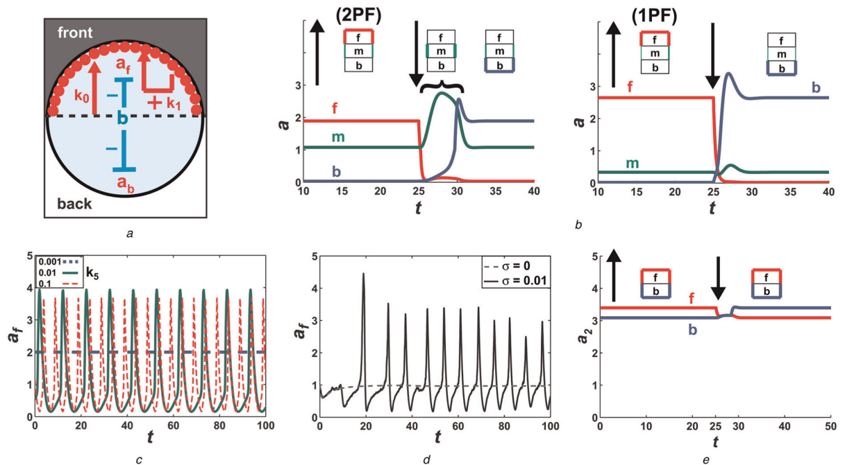
Fig. 2. Compartment modelling of mating morphologies
