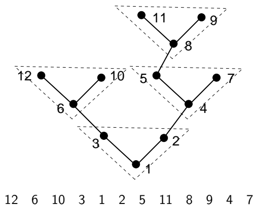
FIGURE 10. The construction of a \mathcal{Y} -permutation enumerated by cm(z) . The elements at even level (underlined) are valleys only.
