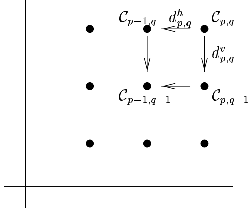
Figure 1.7: Viewing the double complex \mathcal{C}_{**}
