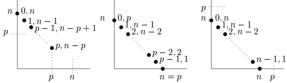
Figure 1.10: Viewing (\mathcal{F}_p \text{Tot}(\mathcal{M}))_n , an object in the subcomplex \mathcal{F}_p \text{Tot}(\mathcal{M})
