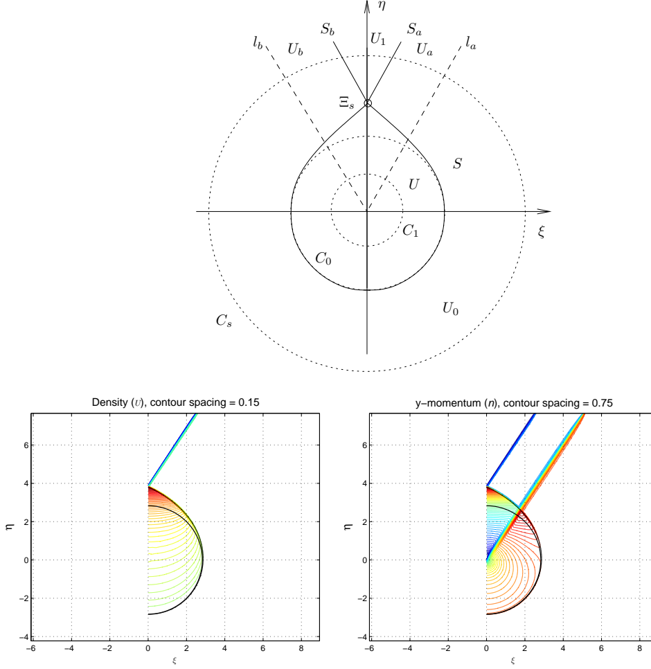
FIGURE 3. Transonic regular reflection for the NLWS: definition of the states (top) and numerical simulation showing the contour plot of \rho (bottom left) and the contour plot of n (bottom right). The inner circle on the bottom figures corresponds to the sonic circle C_0 , and the curve following the reflected wave corresponds to the numerically calculated transition between supersonic and subsonic flow.
