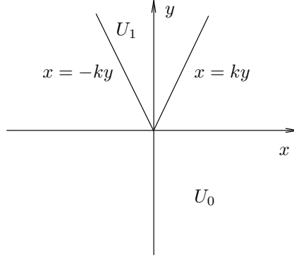
FIGURE 1. The Riemann Initial Data
