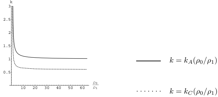
FIGURE 5. The curves k_A and k_C in the (\rho_0/\rho_1, k) -plane for the \gamma -law pressure, \gamma = 2 .
