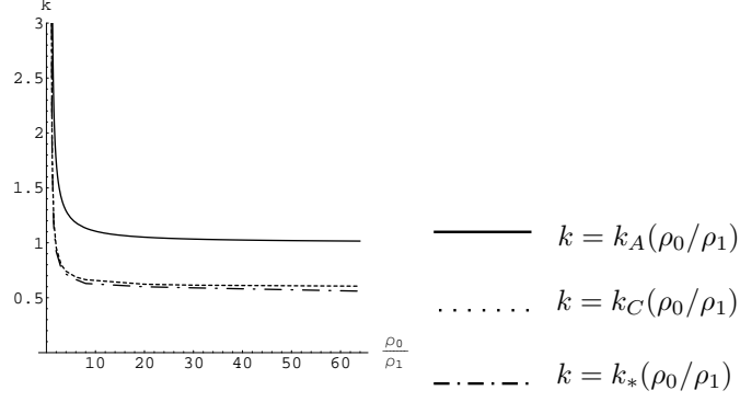
FIGURE 8. The curves k_A , k_C and k_* for the \gamma -law pressure, \gamma = 2 .
