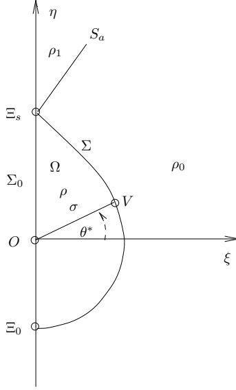
FIGURE 4. The domain \Omega and its boundary.
