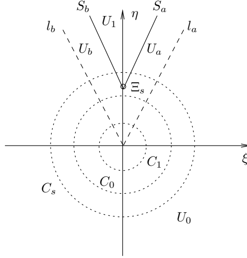
FIGURE 2. Interactions in the hyperbolic region
