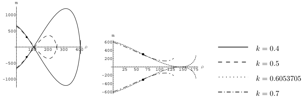
FIGURE 7. The projected shock loci S^+(U_a) and S^-(U_b) in the (\rho, m) -plane for different values of k .
