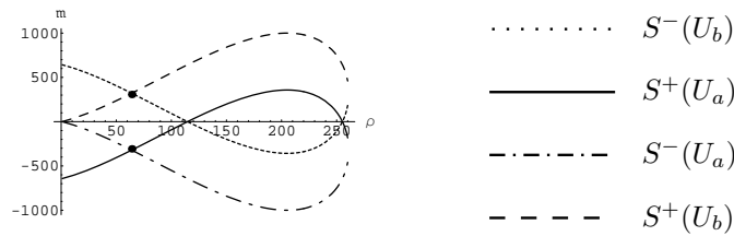
FIGURE 6. The projected shock loci for the states U_a and U_b in the (\rho, m) -plane.
