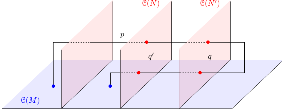
FIGURE 29. A bridge p supported by a mirror M , with subpaths q and q' which are bridges supported by the mirrors N and N' respectively. Notice that only q is a minimal bridge.
