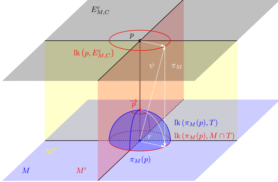
FIGURE 18. Links of points along various subspaces in the proof of Lemma 3.25. Here p is contained in four tiles and sits on the intersection of two mirrors M', M'' . The vertical projection is the nearest point projection \pi_M : E_{M,C}^\varepsilon \rightarrow M .
