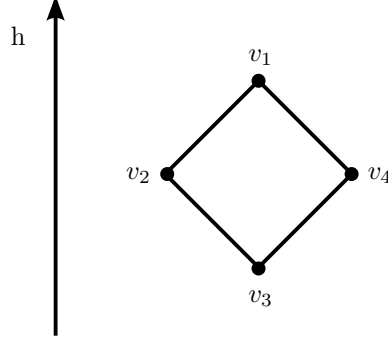
FIGURE 23. A square in \mathcal{C}(\widetilde{X}_\Gamma) .
