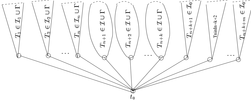
Figure 1: A typical construction of a tree T using a bit B = (\mathcal{I}_1, \mathcal{I}_2, \dots, \mathcal{I}_n; k; \mathcal{I}_0) in a set of bits \mathcal{B} , where t_0 is a new vertex and the summands are from ideals as shown in the figure.
