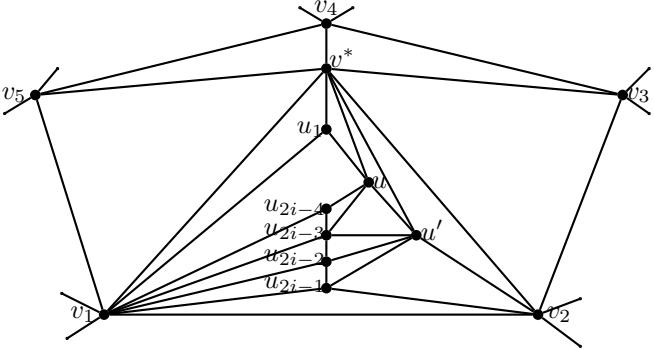
Figure 3: Any graph mapping to infinitely many H_i maps to U' depicted below and U' \leq U .
