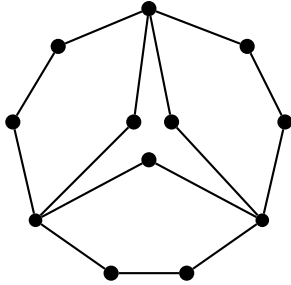
Figure 4: The 3-Pentagon, 3\mathbb{P}
