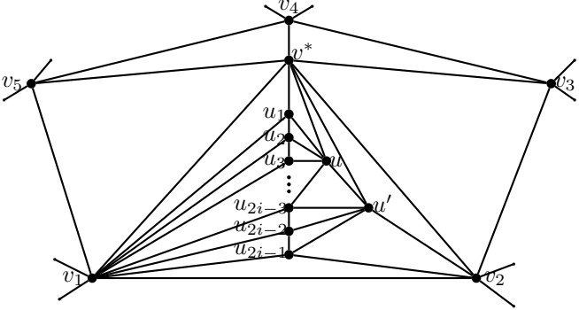
Figure 2: Construction of H_i , by adding vertices u, u' and u_j, j = 1, 2, \dots, 2i - 1 in a face of U , for each i \geq 1
